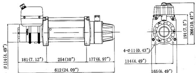
Our TDS-12.0c Goldfish winches are ideal for recovery trucks winching up to 4 tonnes, and heavy off road use. Full of features and are waterproof out of the box.
